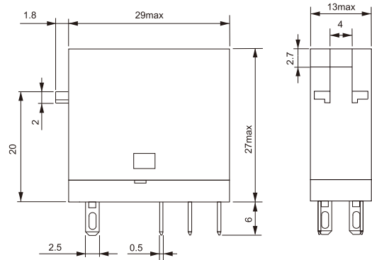
DRPT-2C
