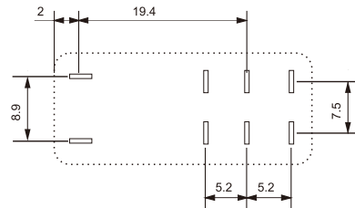
DRPT-2C
