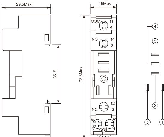
DSRT05A-E3
