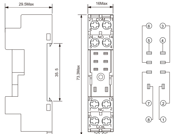
DSRT08A-E3
