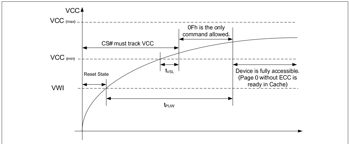
Figure 32 Power-On Timing
