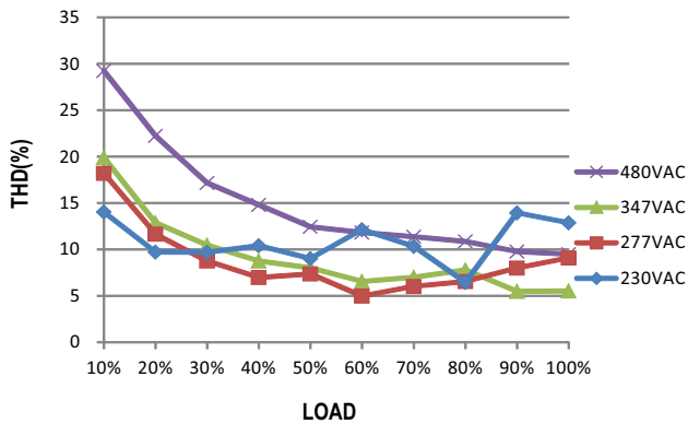
LOAD
