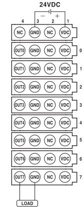
OUT (PNP): 8P, 24VDC 0.3A/Point
