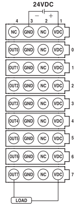
OUT (NPN): 8P, 24VDC 0.3A/Point
