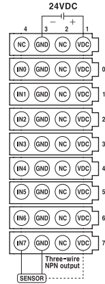
IN (NPN): 8P, 24VDC 10mA
