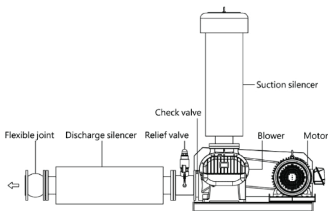
AIR BLOWER
