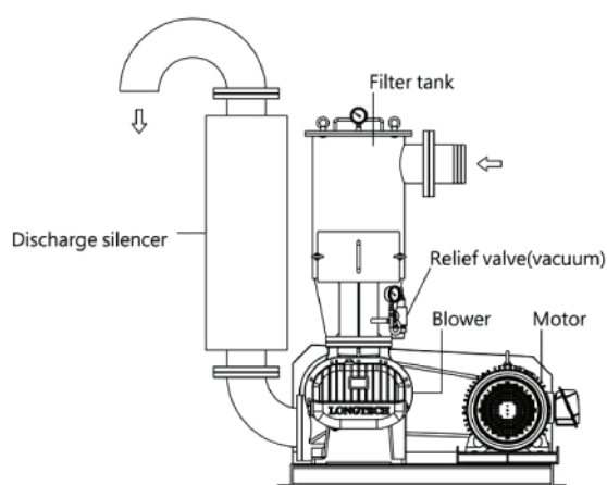
VACUUM PUMP
