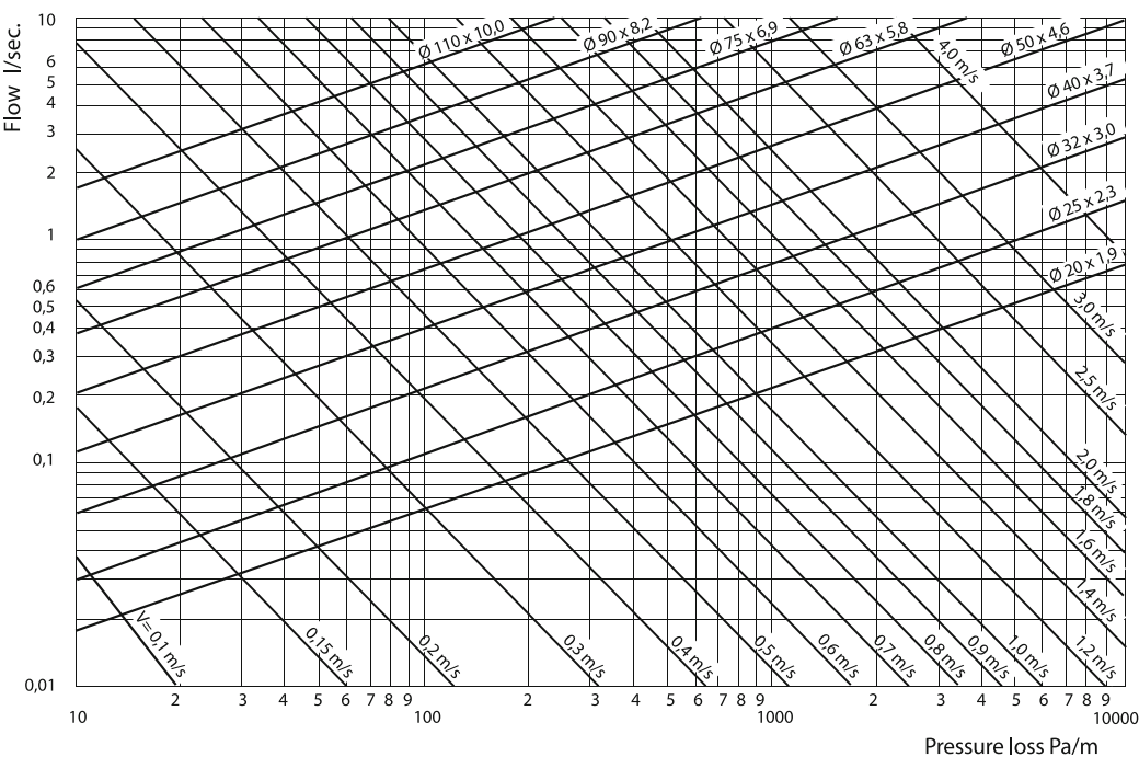
Loss Pressure Diagram for PN10 / PN14 Pipe
