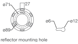
reflector mounting hole
