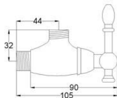
OM-106 Angle Valve RM42
