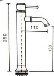
OM50031D Basin Mixer - Tall RM397
