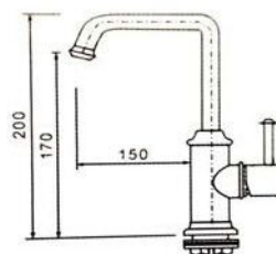
OM50031TA Basin Mixer with Swivel Spout RM343
