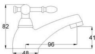
OM-100B Basin Tap RM112
