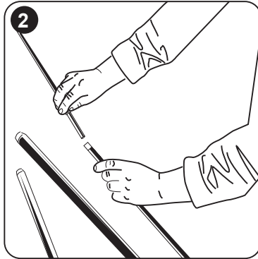
2 Continue joining subsequent thickness Pole sections until the protected end of the Pole has reached the end of the Flag sleeve at the top of the Flag
