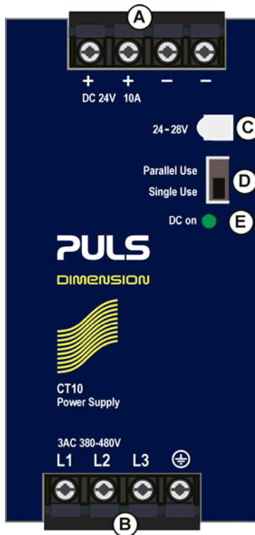
Fig. 10-1 Front side
