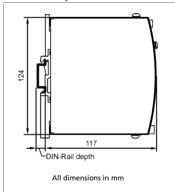
Fig. 20-2 Side view
