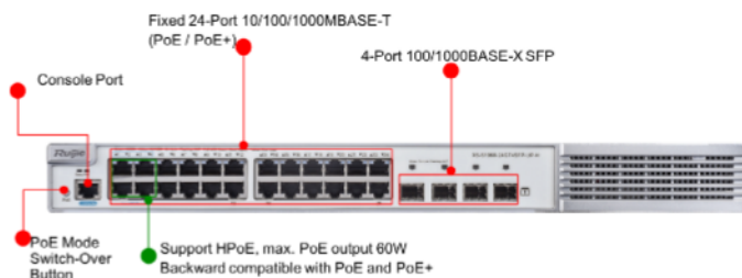
Figure 4: PoE/PoE+ Support
