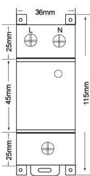
C-240AC Top View
