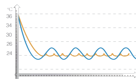
GA Stepless Inverter Mode Ordinary Mode
