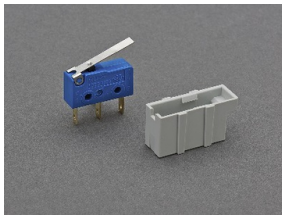
33 917 pilot switch changeover 250 V AC / 5 A; 30 V DC / 4 A Size 1
