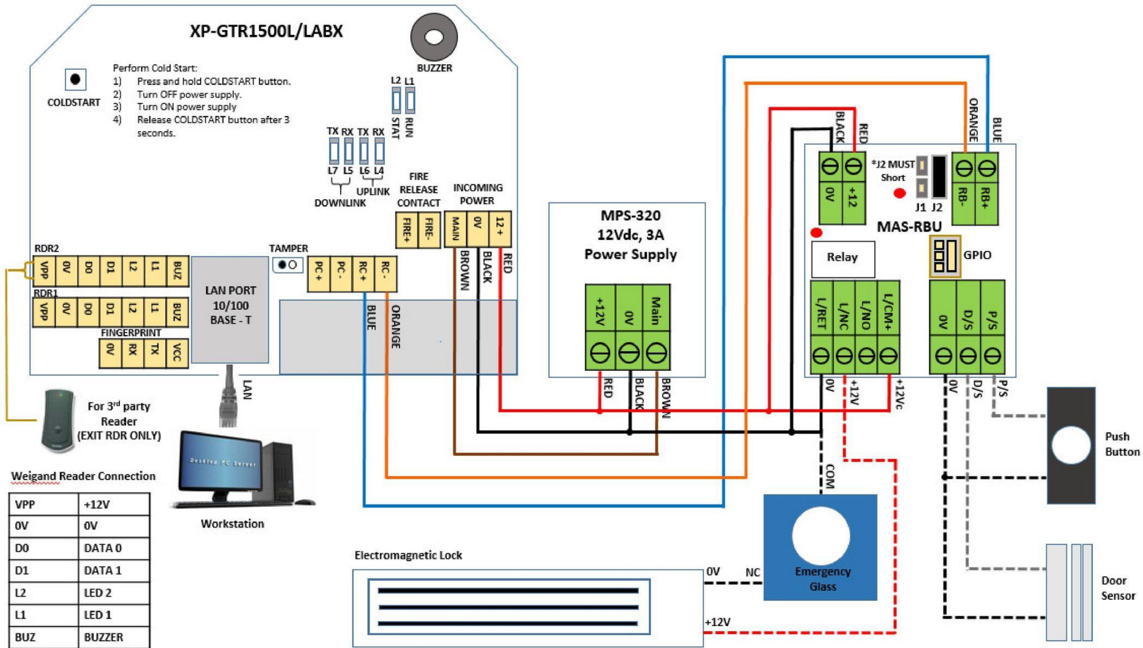
Wiring Diagram : GTR 1500 and Door Accessories with LAN Connection
