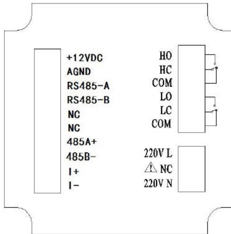
Wiring diagram
