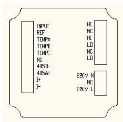
Wiring diagram
