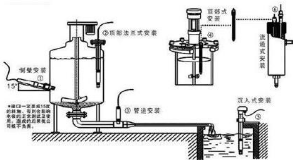
Schematic diagram of common installation method
