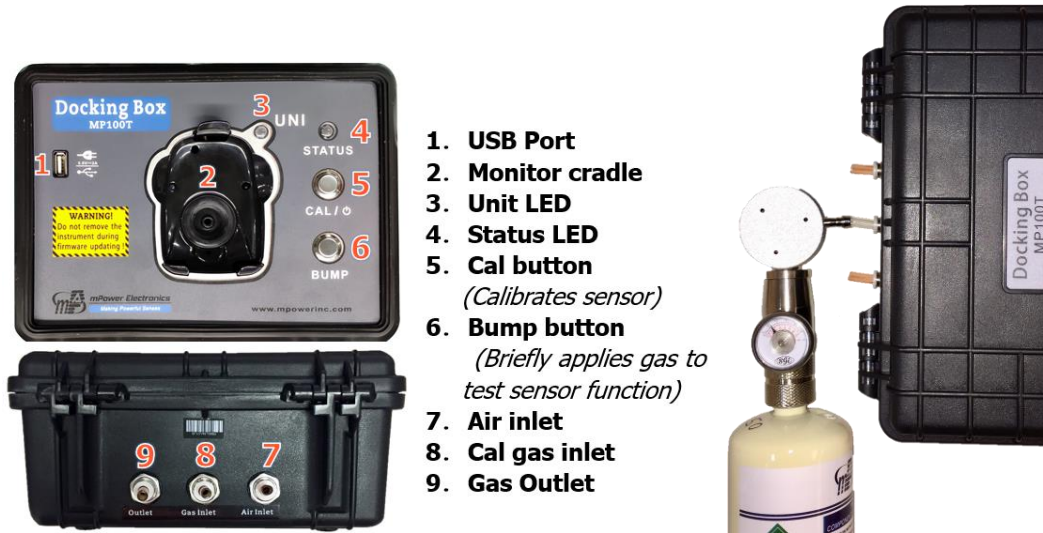
Docking Box Components
