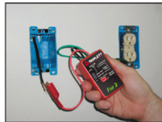
“Line to ground” testing using Alligator clips
