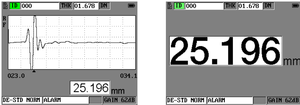
Measure in standard echo detection mode
