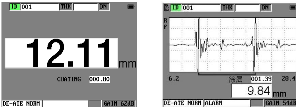
THRU-COAT mode showing the thickness of a coating and steel (waveform not activated)
