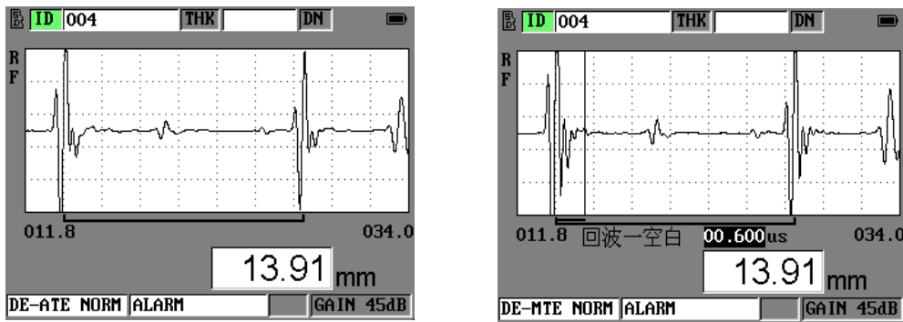
Measurement in automatic E-E detection mode
