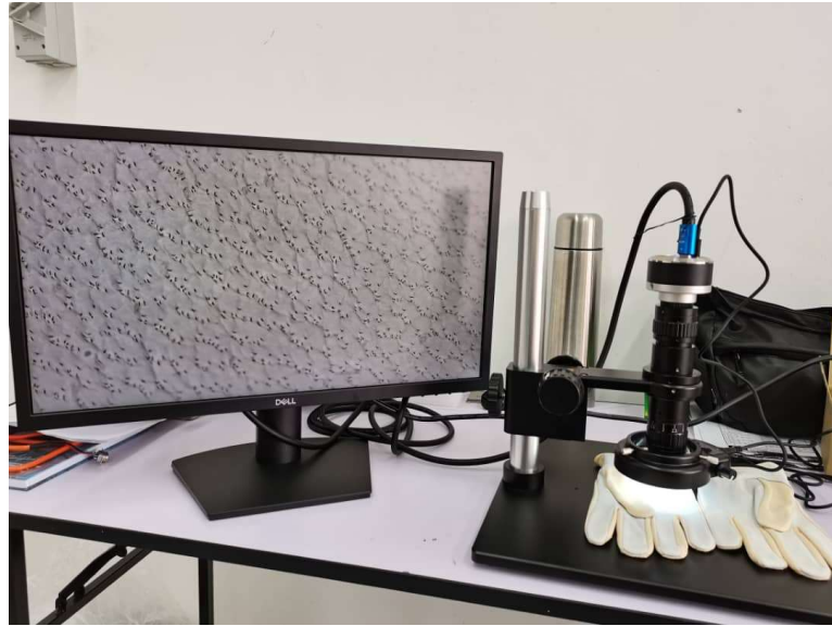
Figure 1.1: Life Image Capture through Digital HD Video Microscope
