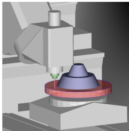
Five-axis to prevent the collision
