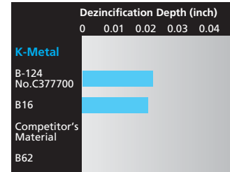
Fig. 4 Comparison of dezincification (to AS C316)
