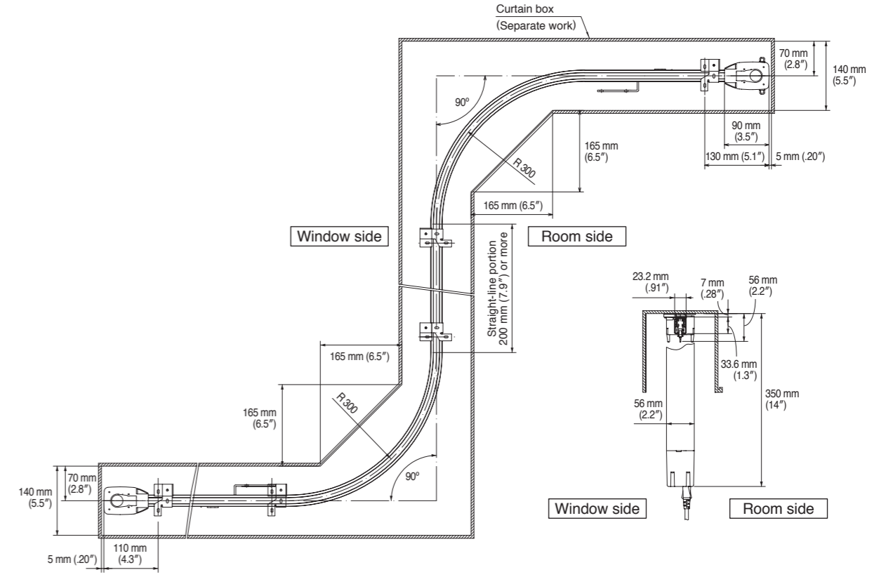
Two curves (S-shaped): ceiling single attachment
