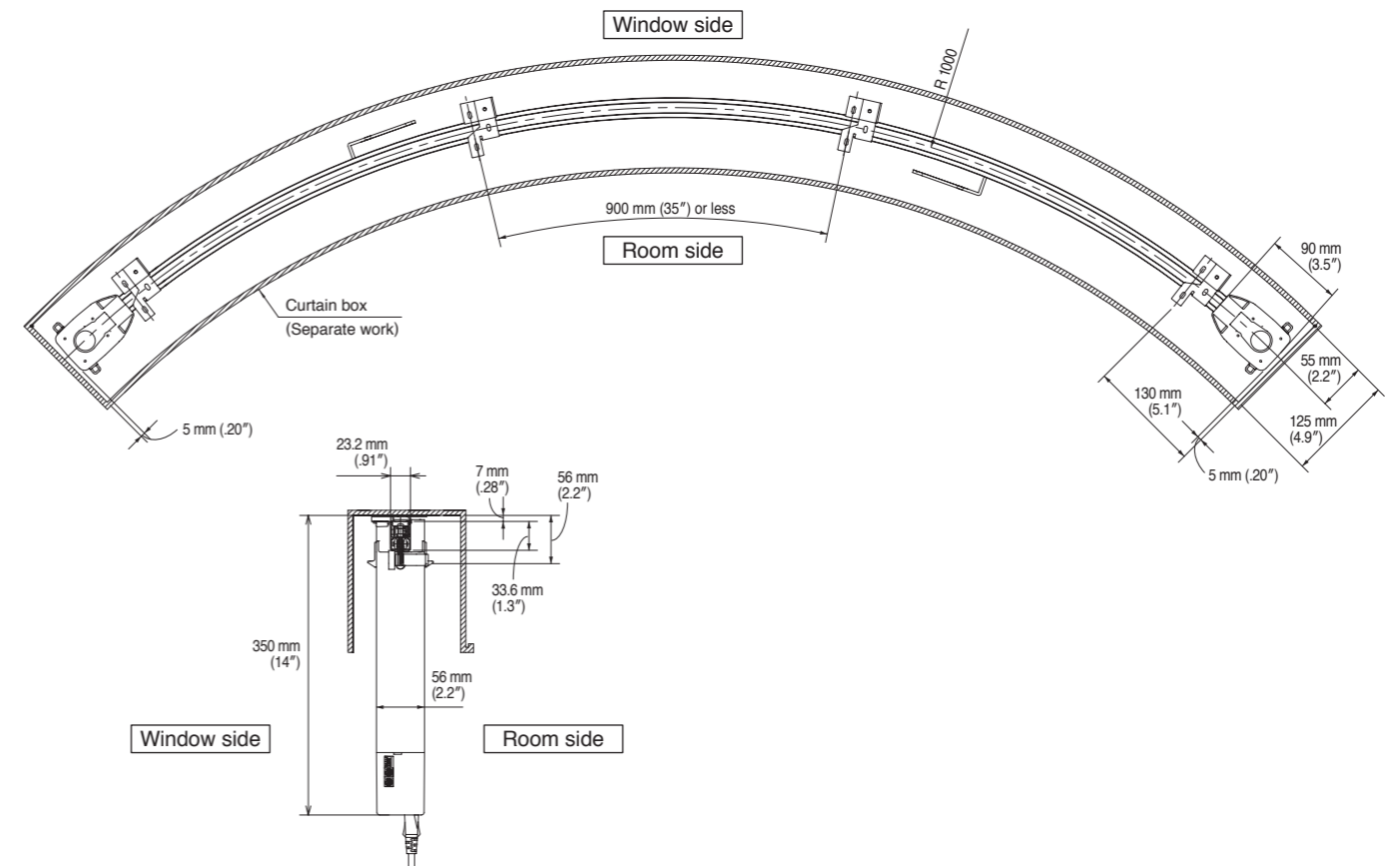
Gradual curve: ceiling single attachment
