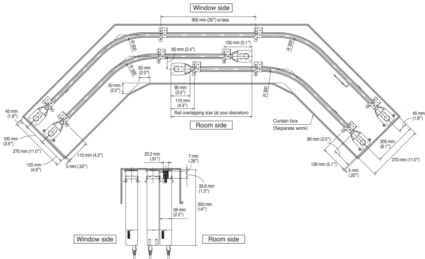
Two curves: ceiling single attachment (Room side: Overlap with two rails, Window side: Master roller)
