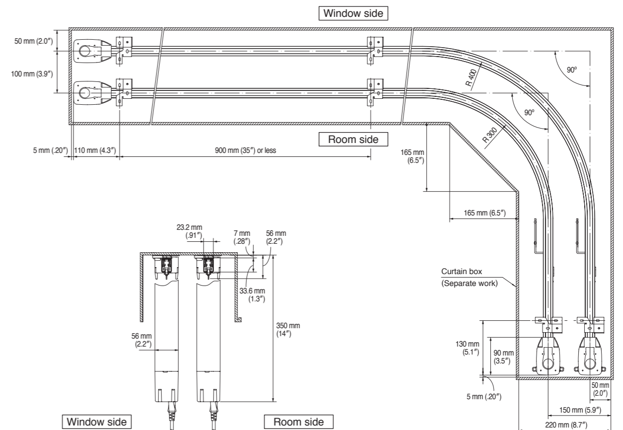
Single curve: ceiling double attachment
