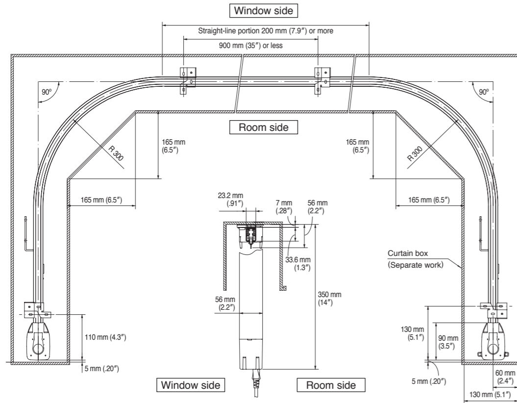
Two curves: ceiling single attachment
