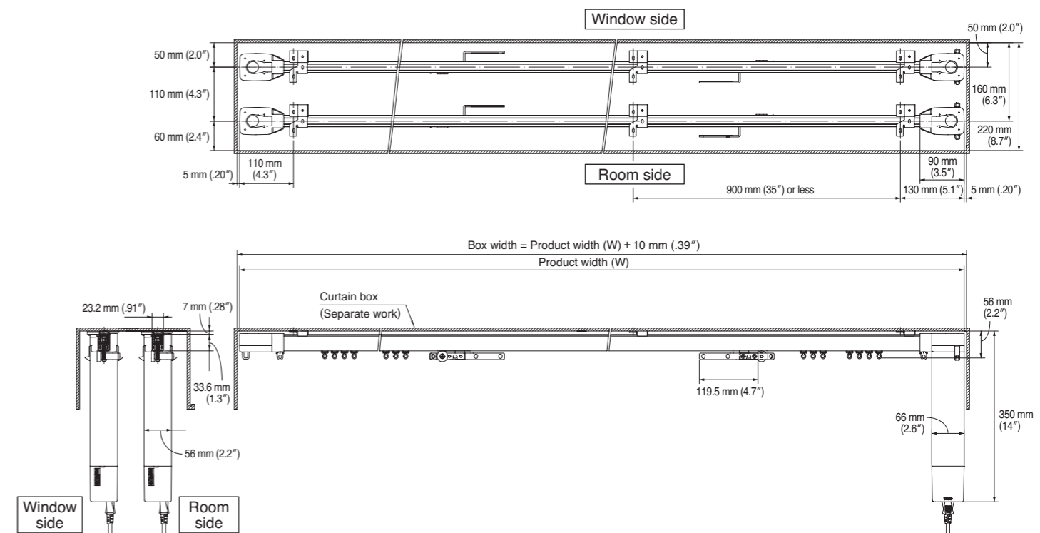
Two-way draw: ceiling double attachment
