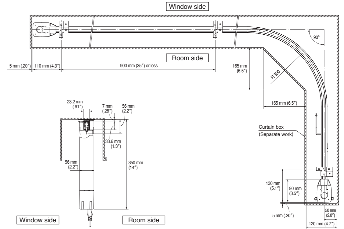
Single curve: ceiling single attachment
