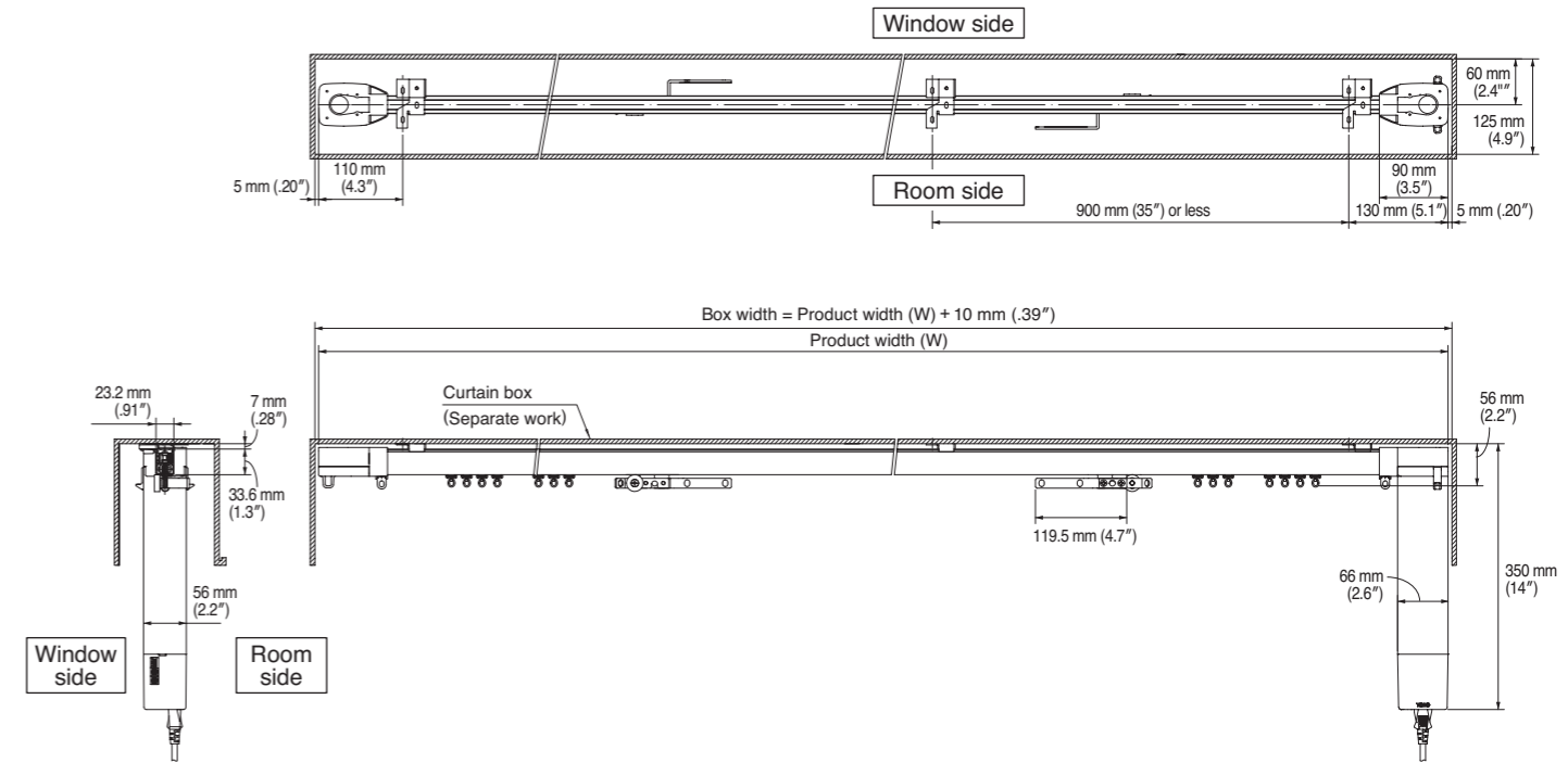
One-way draw: ceiling single attachment
