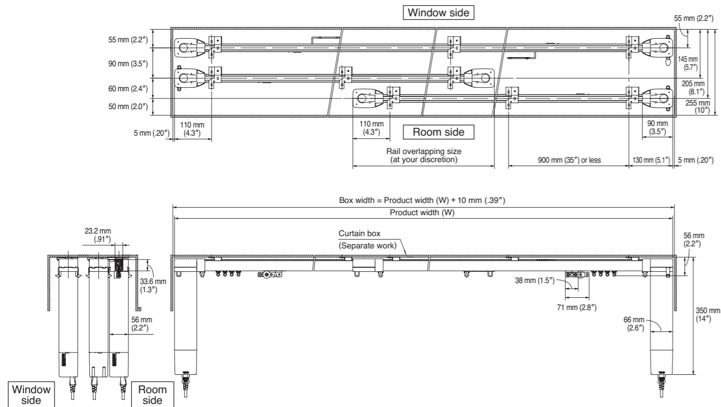
Two-way draw: ceiling double attachment (Room side: Overlap with two rails, Window side: Master roller)
