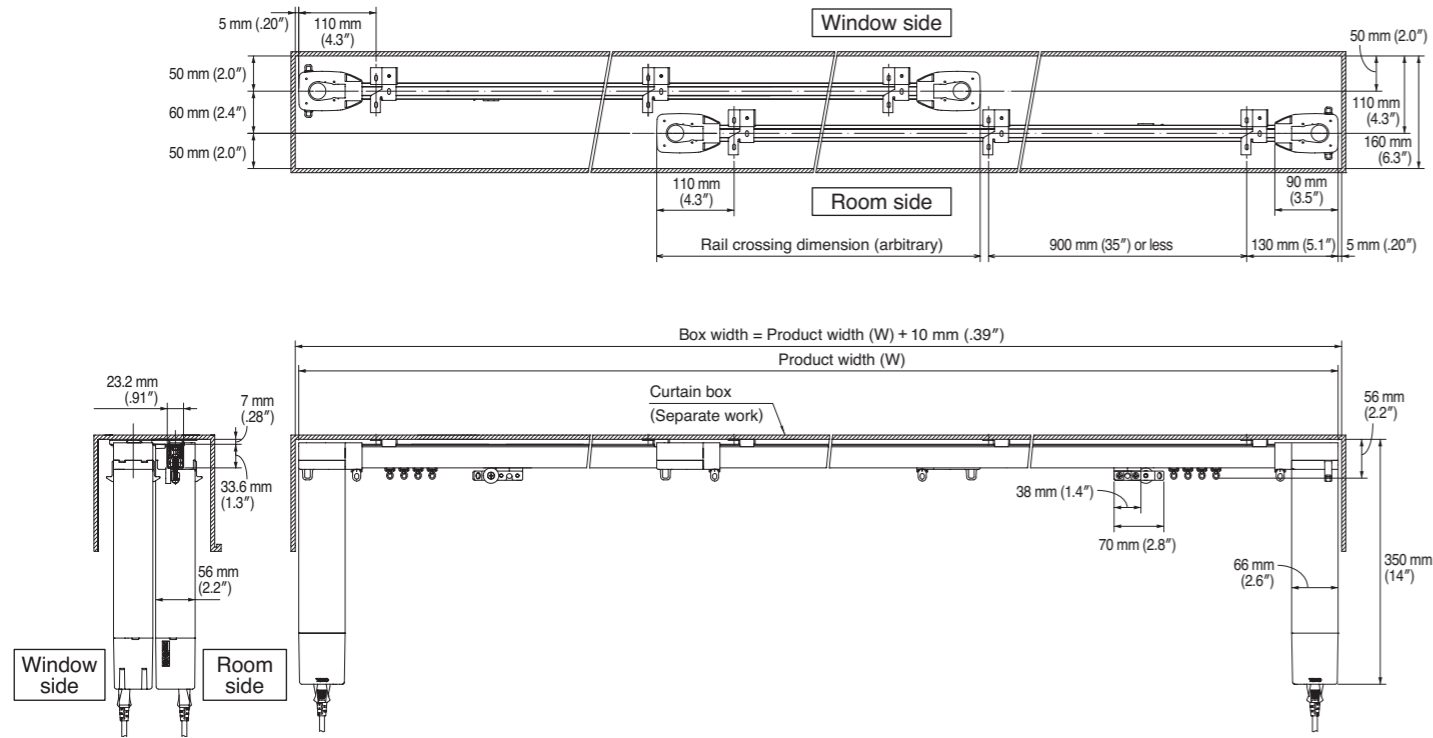
Two-way draw: ceiling single attachment (Overlap rail)
