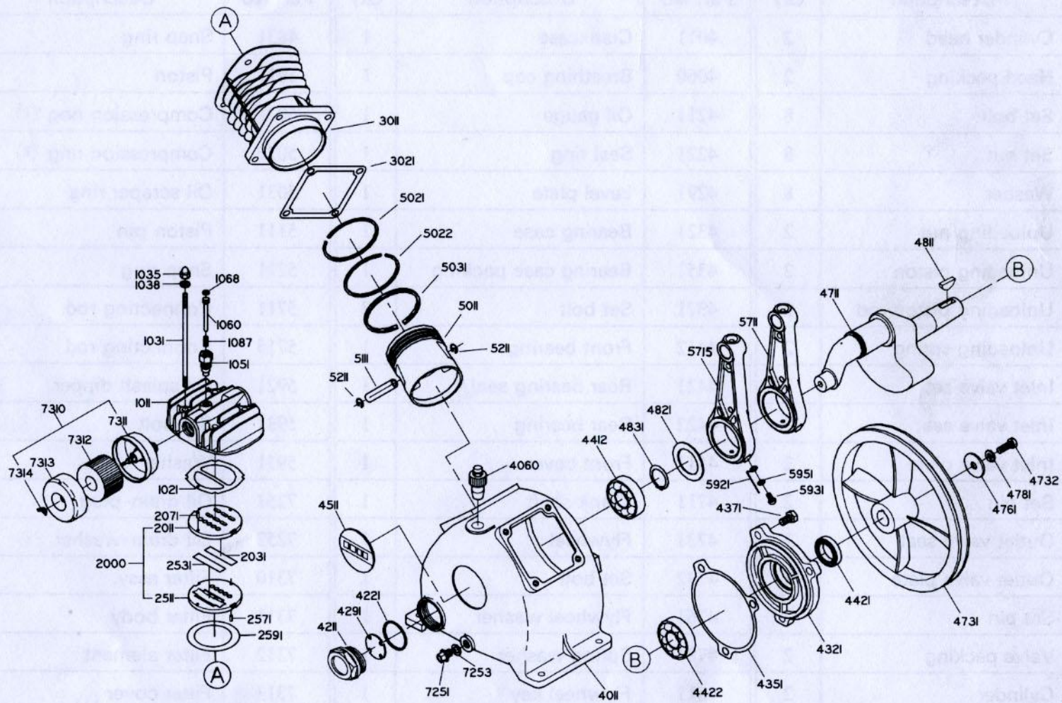
SVU(P)-201(202) COMPRESSOR BODY
