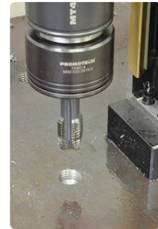
Tapping tool
