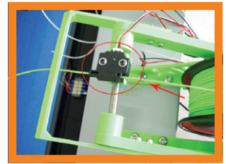
Material Broken / Finish Detector
