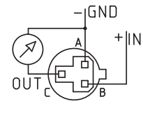
B (IN) C (OUT) A (GND)
