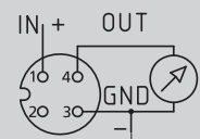
1 (IN) 3 (GND) 4 (OUT)
