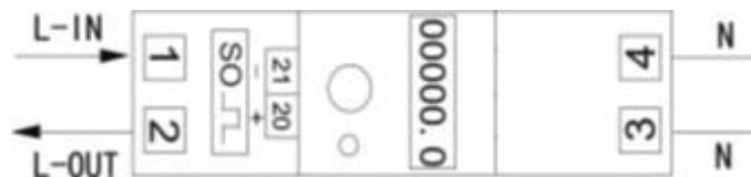
Connection Diagram
