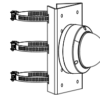
DS-1275ZJ-SUS Vertical Pole Mount
