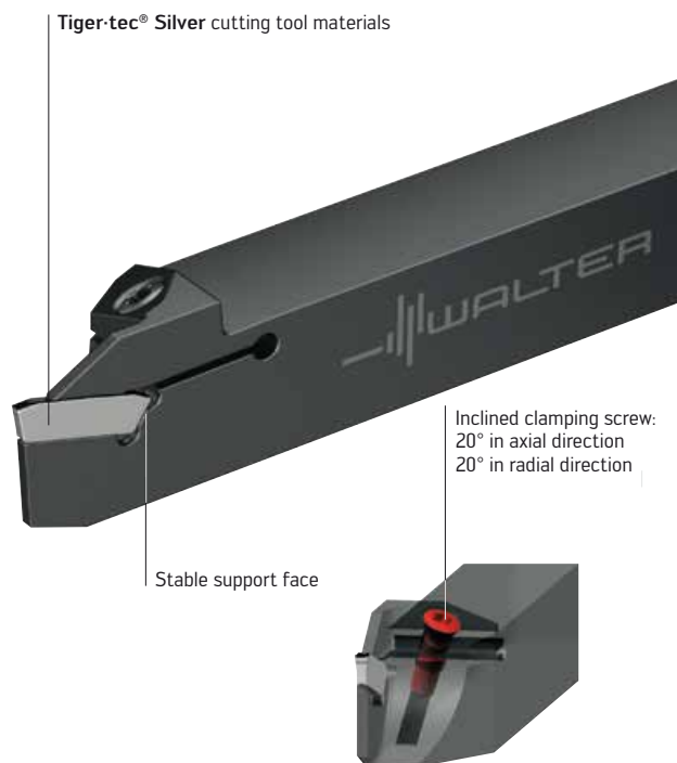
Walter Cut monoblock toolholder
