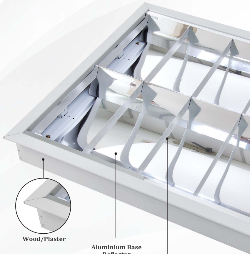
Aluminium Louvre
