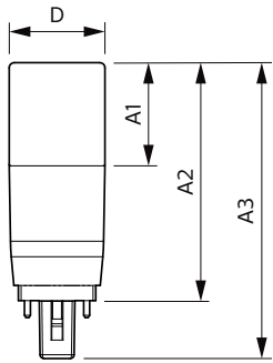
LED PLC 9W 840 2P G24d
