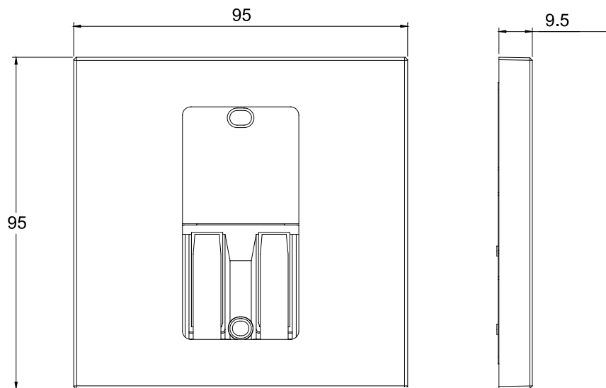
Frame Dimensions
