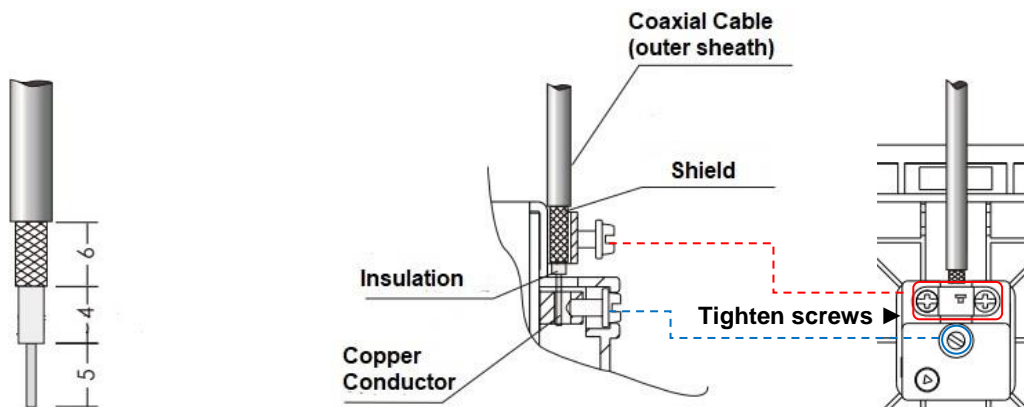
Cable strip lengths (mm)
