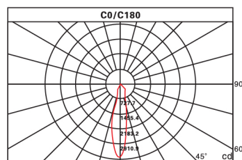
Lux-Distance Curve
