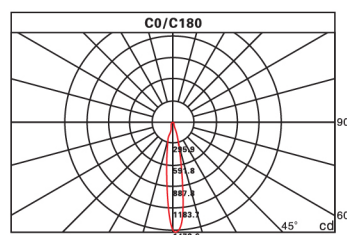
Lux-Distance Curve
