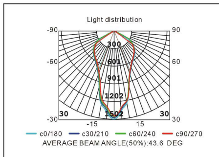
Light Distribution
