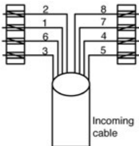
RJ45 Jack
