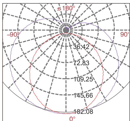
cd/klm 100% — C0 - C180 — C90 - C270
