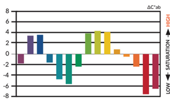
Conventional LED CRI 70
