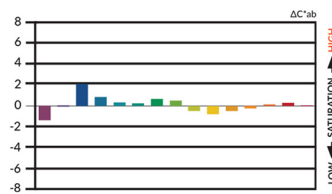
High CRI LED CRI 80
