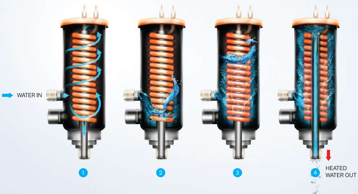
WATER HEATING PROCESS OF UL-APPROVED HIGH QUALITY UK TECHNOLOGY HEATING ELEMENT
