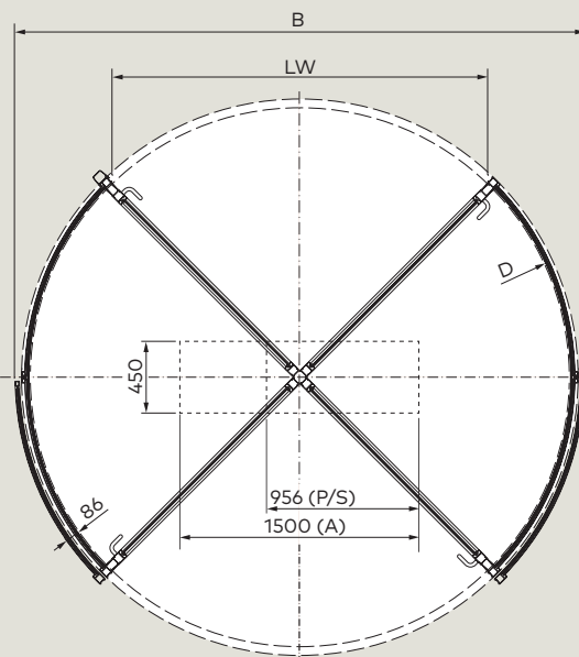
Drum wall with safety glass
