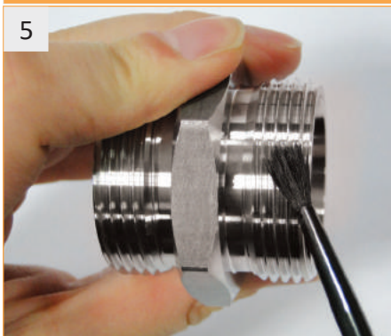
Lubricate thread and cone of fitting body, also compression ring and thread of nut.
