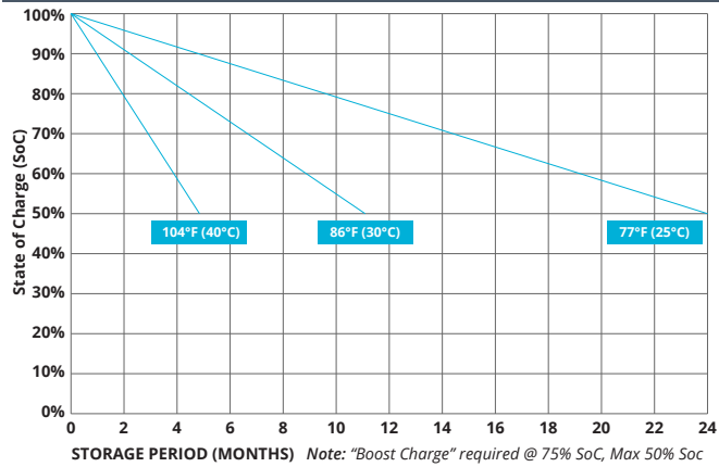
SELF DISCHARGE vs TIME/TEMPERATURE
