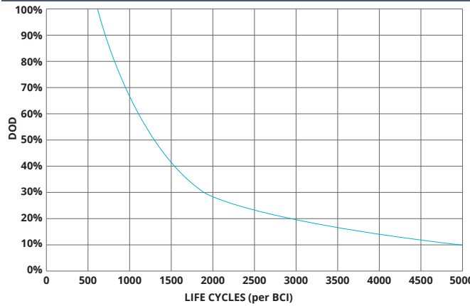
CYCLE LIFE vs DEPTH of DISCHARGE (DOD) *(Based on BCI Testing @ 2-hr Rate)
