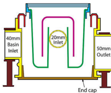
SPIND Mini Side Flow c/w 2 inch outlet for fully cast in concrete slab design
