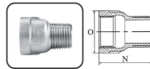
SOCKET M/F FIG NO. 11
