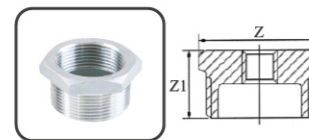
RED. HEXAGON BUSH FIG NO. 18
