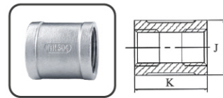
SOCKET BANDED FIG NO. 9
