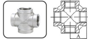
CROSS TEE FIG NO. 2
