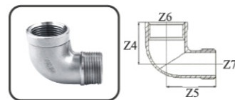
RED. STREET ELBOW FIG NO. 20
