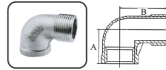
STREET ELBOW FIG NO. 4
