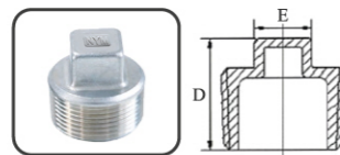
SQUARE PLUG FIG NO. 6
