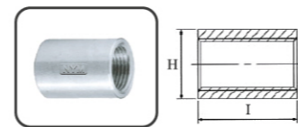
FULL COUPLING FIG NO. 8
