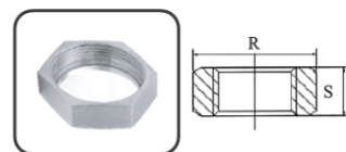
HEXAGON LOCK NUT FIG NO. 13
