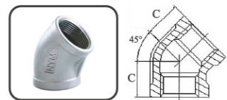
45° ELBOW FIG NO. 5
