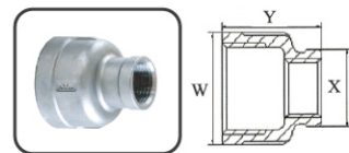
REDUCING SOCKET FIG NO. 17
