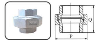
UNION FIG NO. 12
