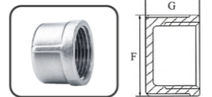
ROUND CAP FIG NO. 7
