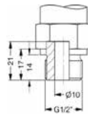
G1/2" DIN 3852 open pressure port 4
