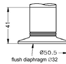
clamp 1 1/2" ISO 2852 (P_N \leq 16 bar)
