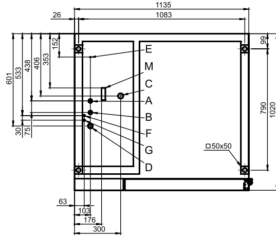
Connection positions
